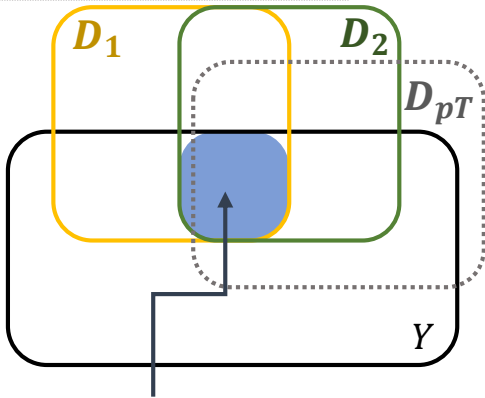
Domain-Invariant Representation
